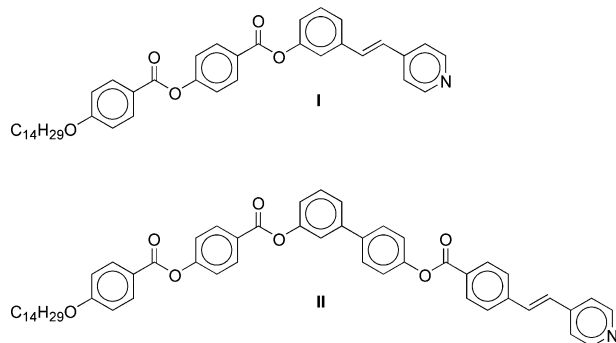
Figure 2. Chemical structures of the H-acceptors used in a previous study.
