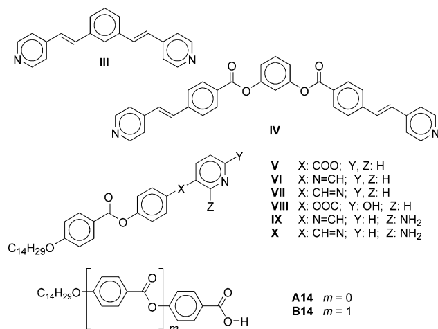
Figure 3. Chemical structures of the H-acceptors and H-donors used in this work.
