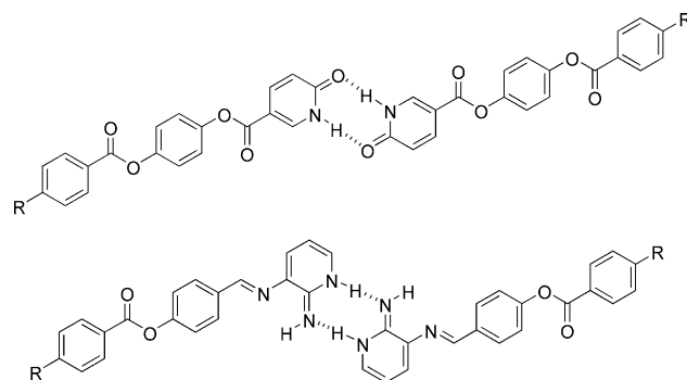
Figure 8. Chemical structure proposed for the dimers formed for compounds VIII and X in the condensed phases.
