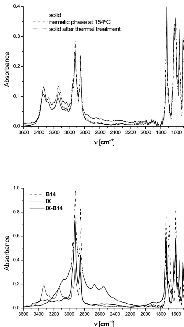
Figure 7. IR spectra (KBr) of compound IX at different temperatures (top) and that of complex IX-B14 and its components ( B14 and IX ) at room temperature (bottom).
