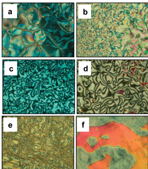
Figure 4. (a) Complex IV-B14 at 178 °C in the SmC mesophase; (b) complex VII-B14 at 119 °C, showing the transition from the N to the SmC phase on cooling; (c) complex VI-B14 at 144 °C in the N mesophase; (d) complex V-B14 at 145 °C in the N mesophase; (e) complex IX-B14 at 112 °C in the SmCP phase; (f) complex IX-B14 at 135 °C in the N phase.
