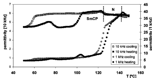
Figure 12. Temperature behaviour of the dielectric permittivity for complex IX-B14 .
