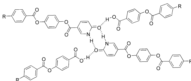
Figure 9. Chemical structure proposed for the material afforded by mixing VIII and B14 .
