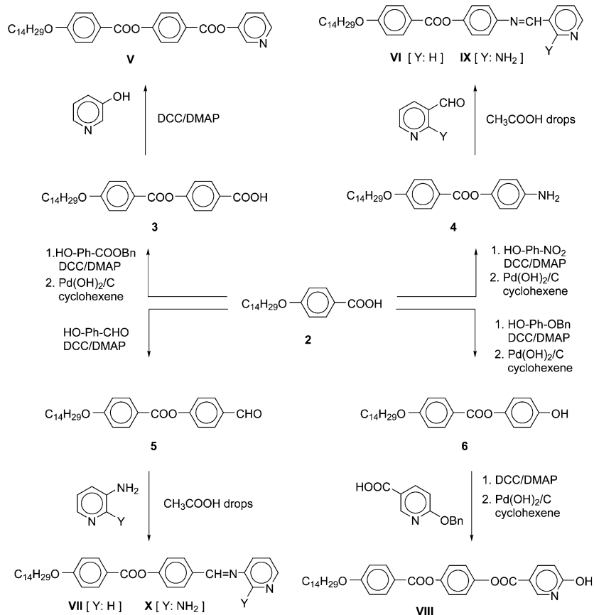
Scheme 2. Routes for synthesis for compounds V–X .
