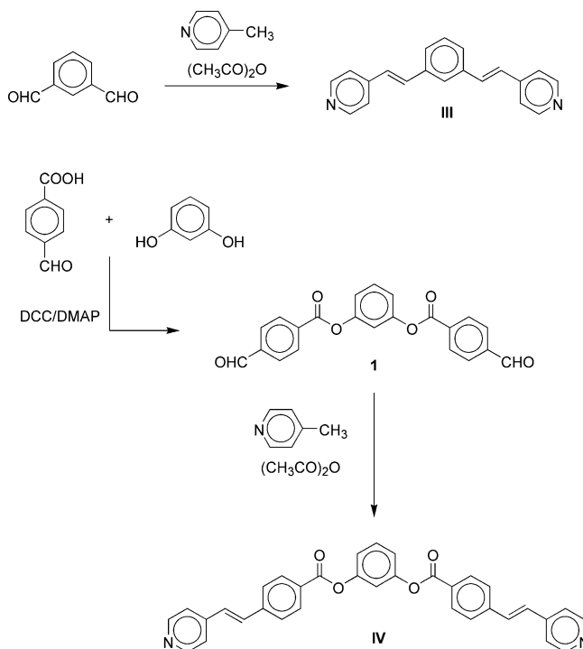
Scheme 1. Routes for synthesis for compounds III and IV .
