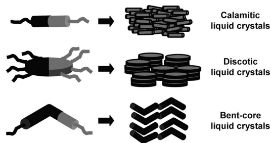
Figure 1. Different liquid crystals generated by using H-bonds.
